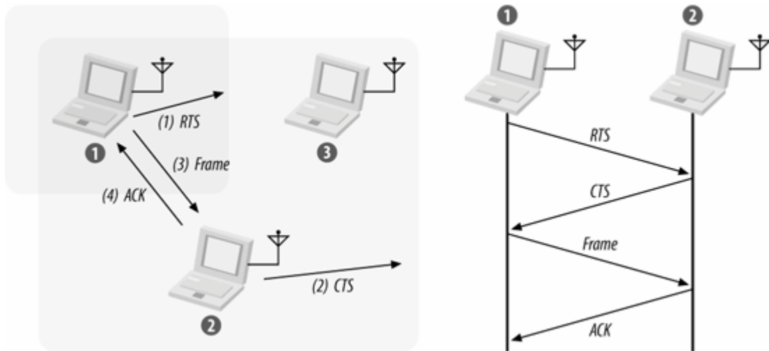
Figure 3-3. RTS/CTS clearing
