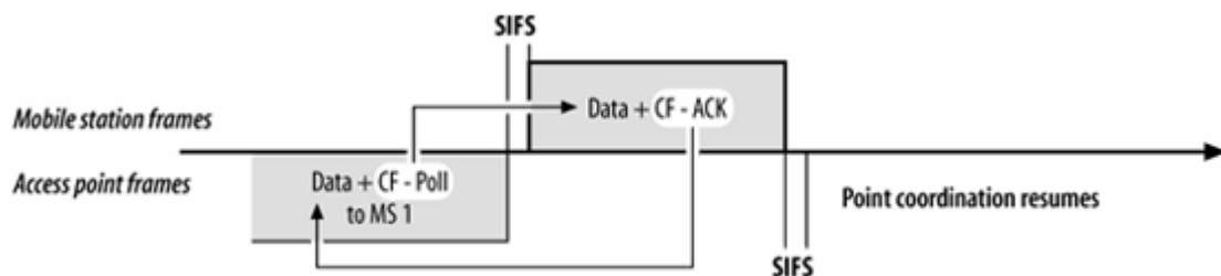
Figure 9-3. Data+CF-Ack usage
