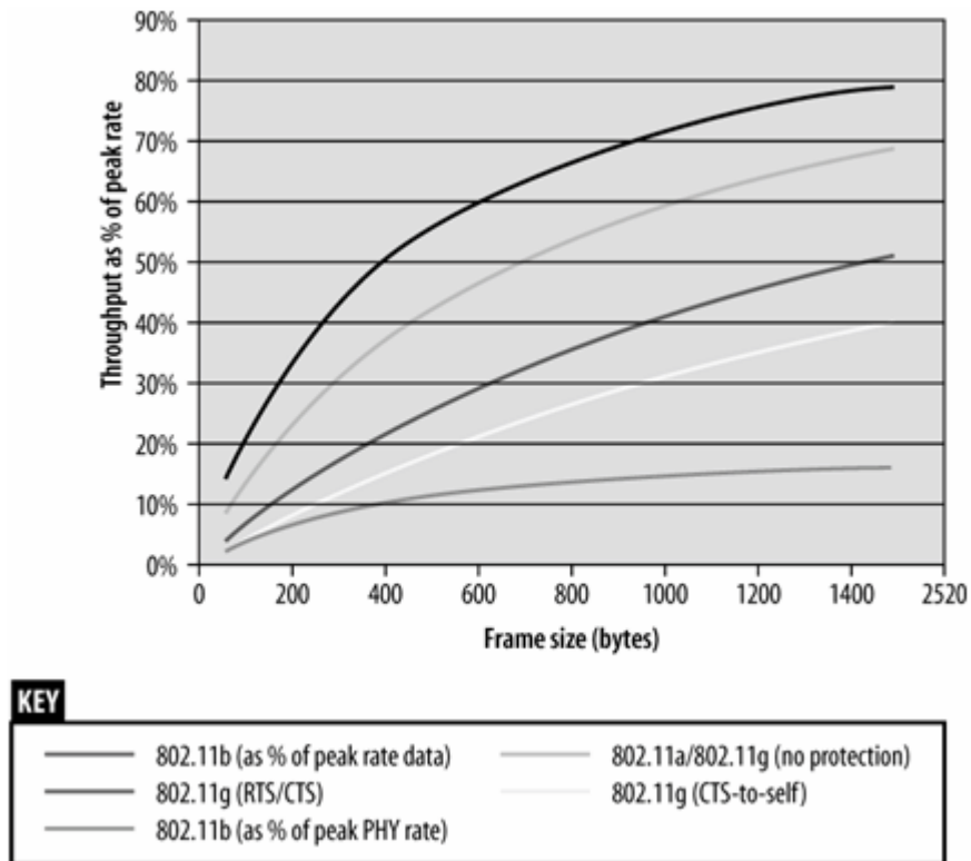
Figure 15-1. MAC Efficiency
