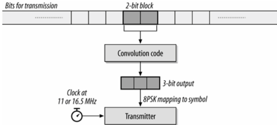
Figure 14-6. PBCC processing
