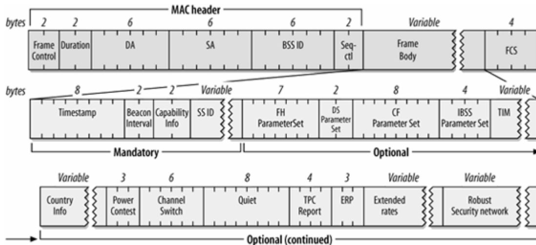
Figure 4-51. Beacon frame
