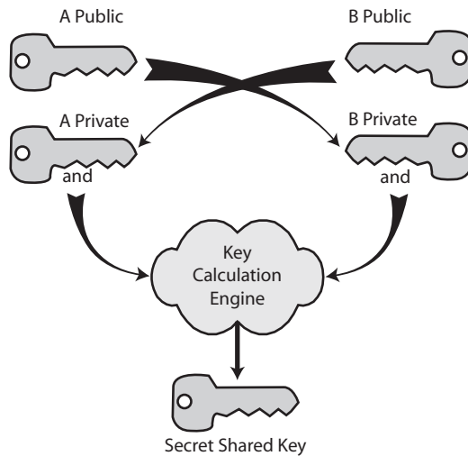
FIGURE 3.2 Diffie-Hellman calculation.
