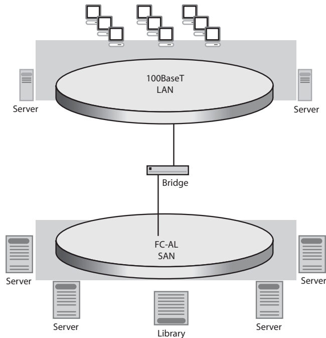
FIGURE 5.4 A storage area network using serverless backup. (© Copyright 2002, StorNet. All rights reserved.)
