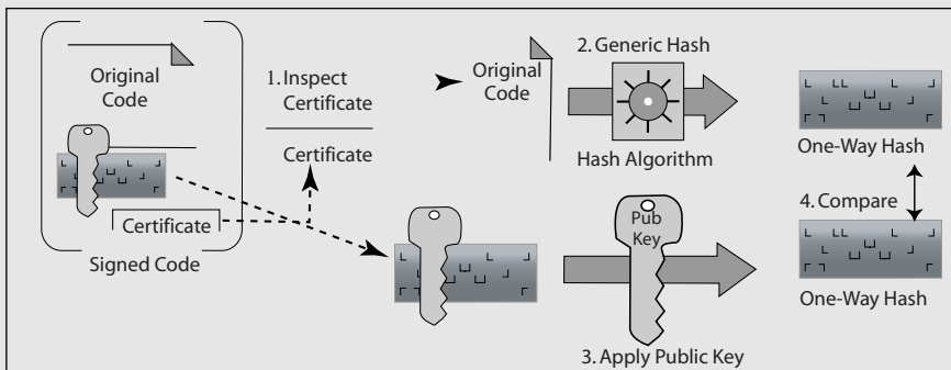
FIGURE 8.4 Authenticode: VeriSign Digital ID process.
