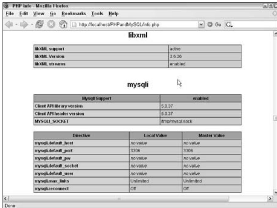
Figure 2-4: MySQL settings.
