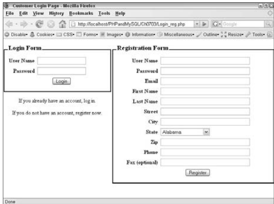
Figure 3-1: The login Web page.
