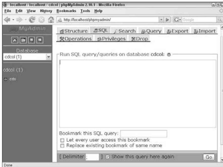
Figure 1-3: The phpMy Admin page that allows you to type an SQL query.
